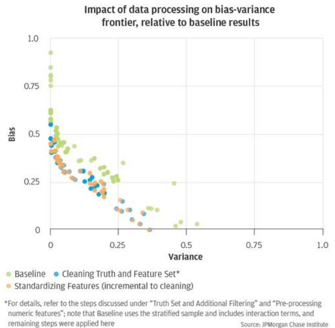
Figure 15 - Model training bias-variance trade-offs
